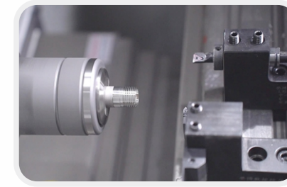
High-precision spindle
