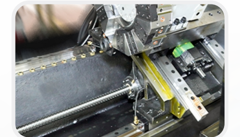
Large diameter high-speed silent ball screw,and roller guide way.
